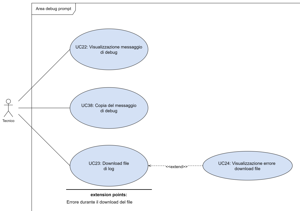
Figura 3.22: Diagramma area debug prompt
